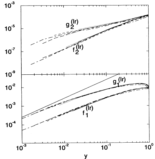
FIG. 6. Scaling functions f_1^{(lr)}(y) , f_2^{(lr)}(y) , g_1^{(lr)}(y) , and g_2^{(lr)}(y) [see Eqs. (6), (8), and (9)] for the mean and variance of the lower and upper bounds, averaged over 1000 realizations of randomness, for t = 256 (solid), 512 (dotted), 1024 (dashed), and 2048 (long dashed). The straight line has slope 1.
