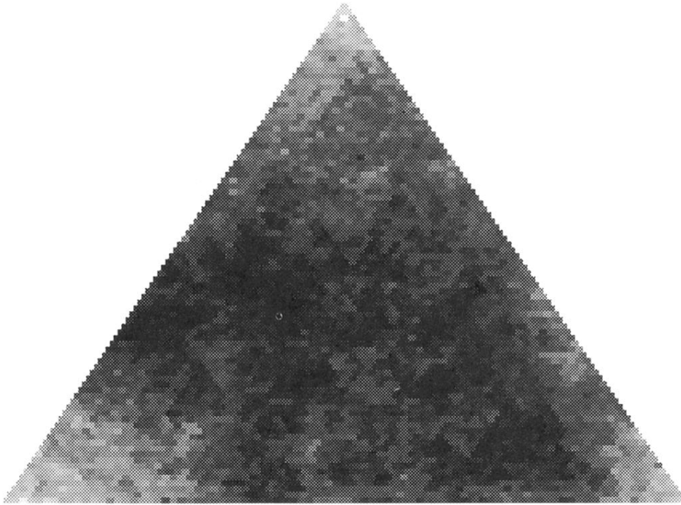
FIG. 8. Minimal energies of paths of length t = 288 in three dimensions to end points \vec{x} with |\vec{x}| < O(t^{\zeta}) . The higher energies are indicated by white shading, and the lower energies by darker shades.
